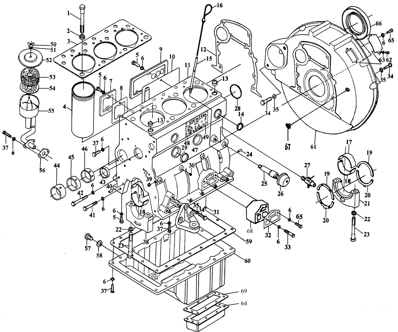
Fig. 1 Engine Body Assy(Y385 T-1)
