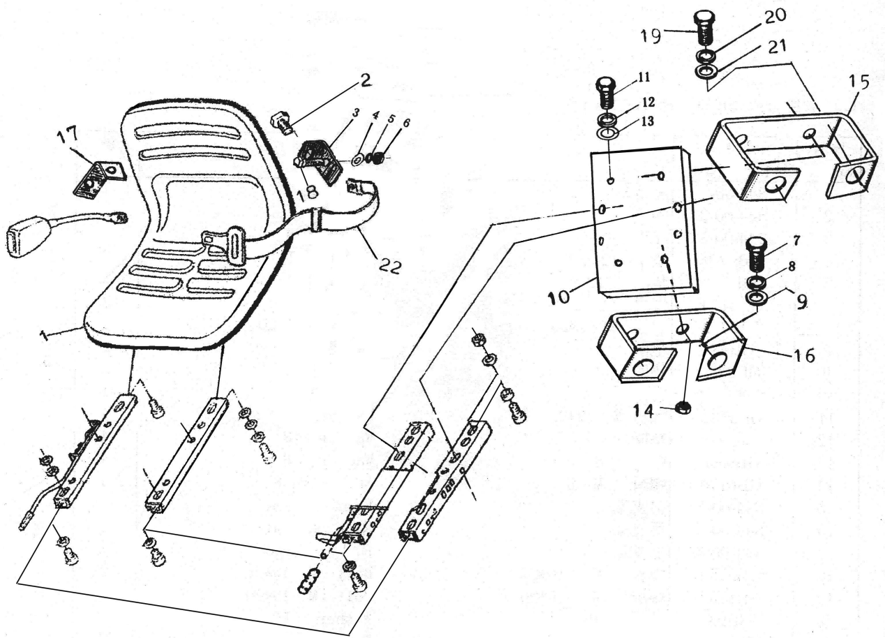
Fig. 13 Seat
