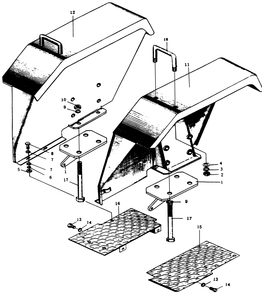
Fig.15 Mud Shield And Step
