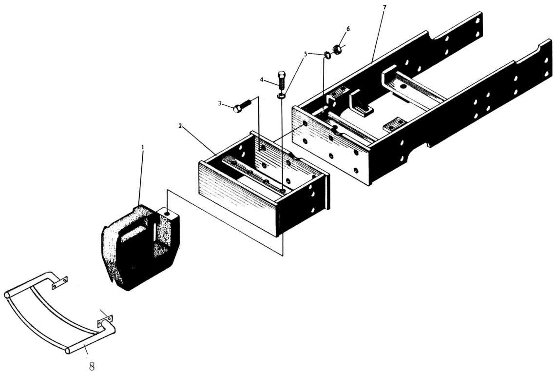
Fig. 16 Bracket
