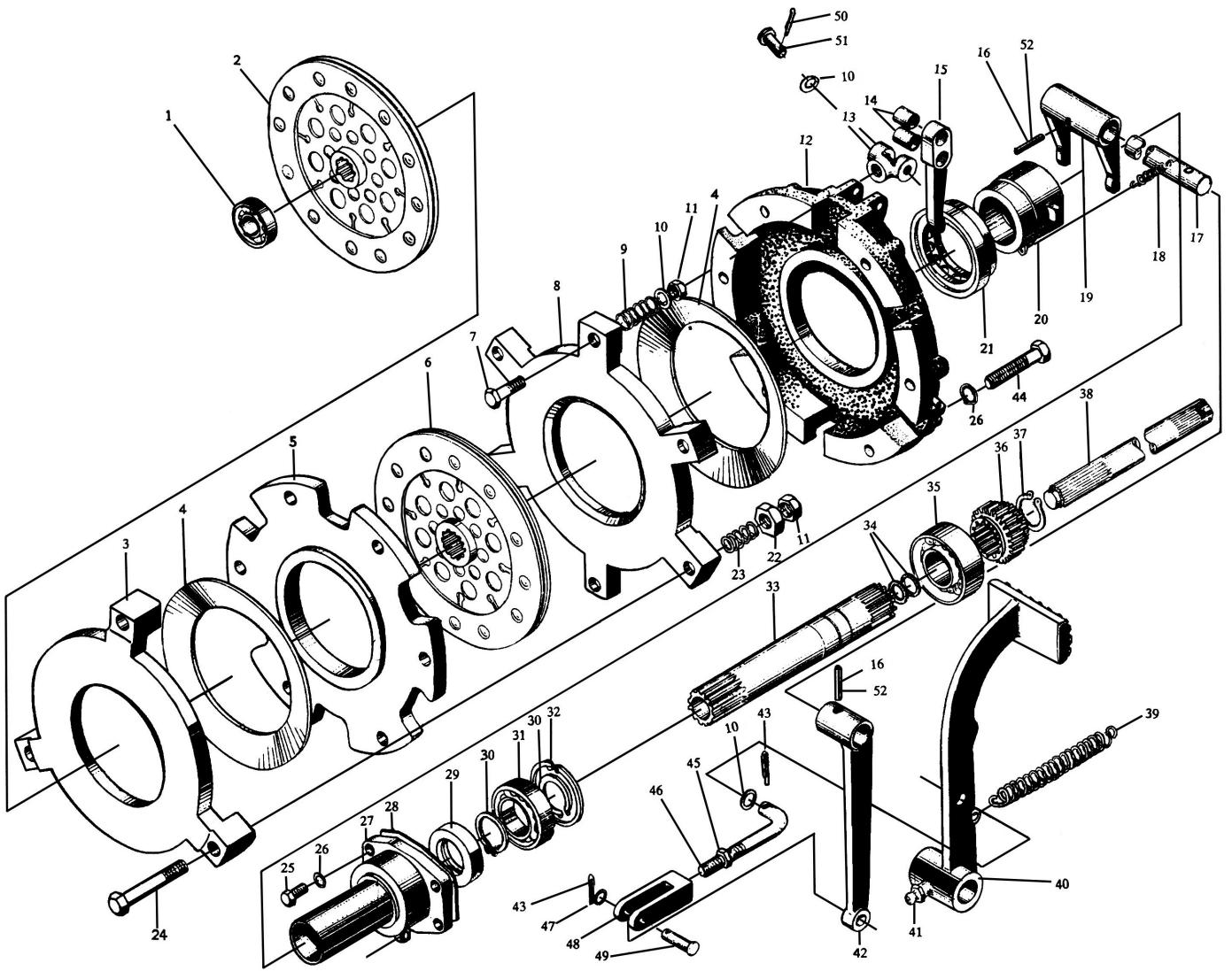
Fig.2 Dual Stage Clutch
