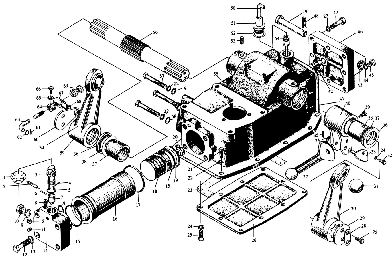
Fig.20 Hydraulic Power Lift
