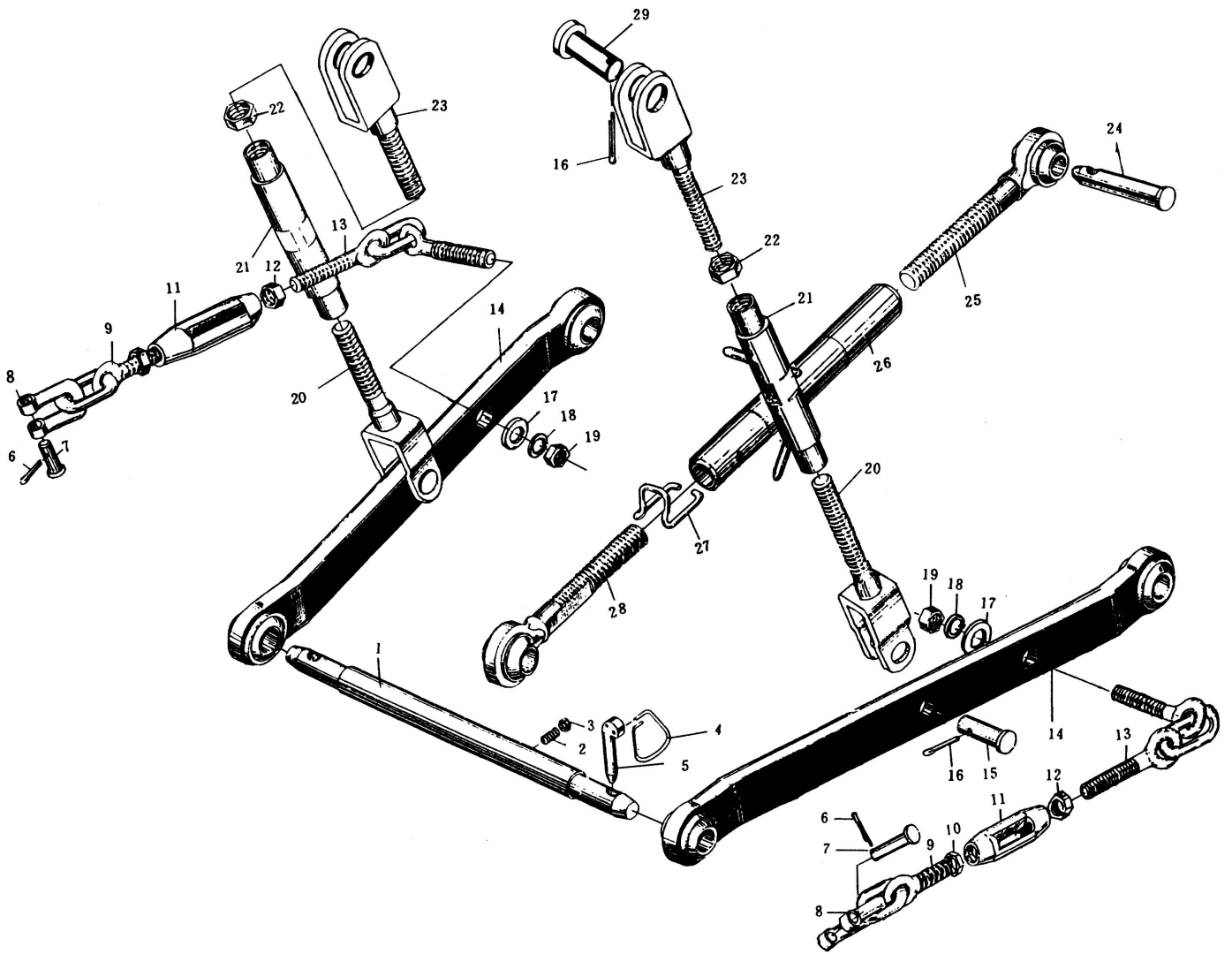
Fig. 21 Suspension Mechanism II
