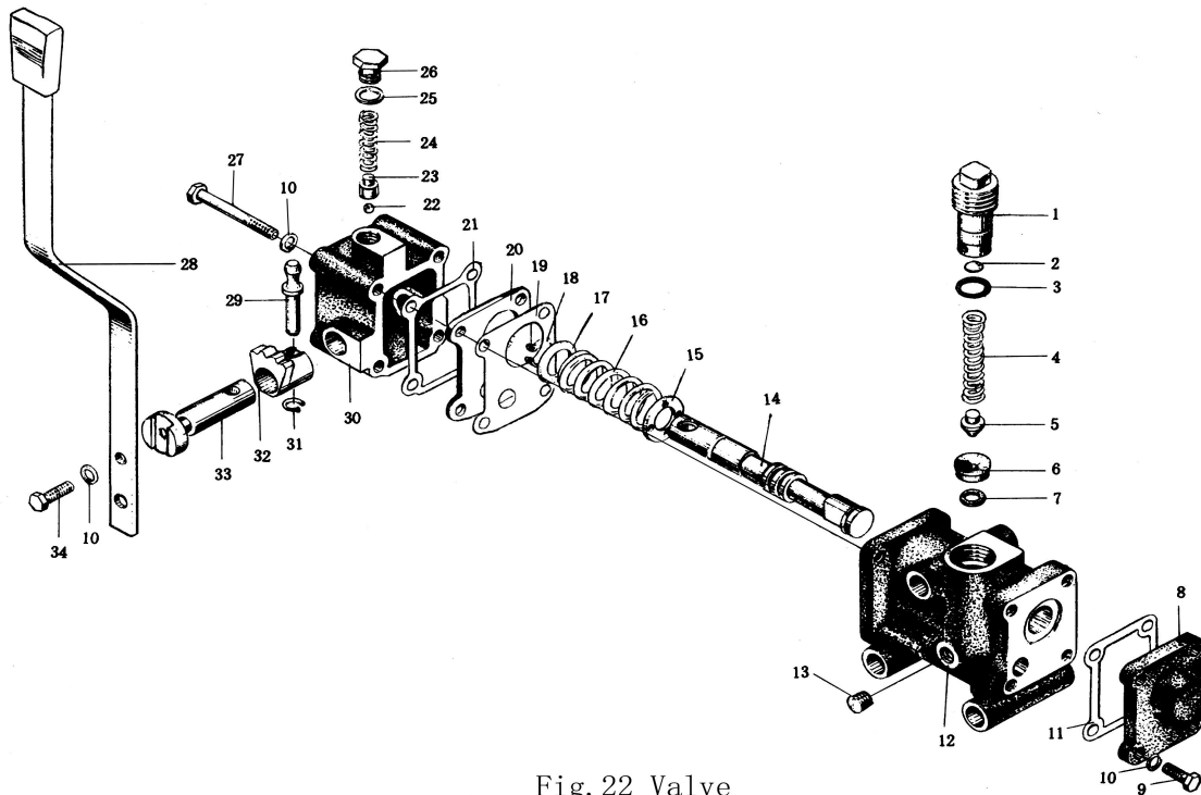
Fig. 22 Valve
