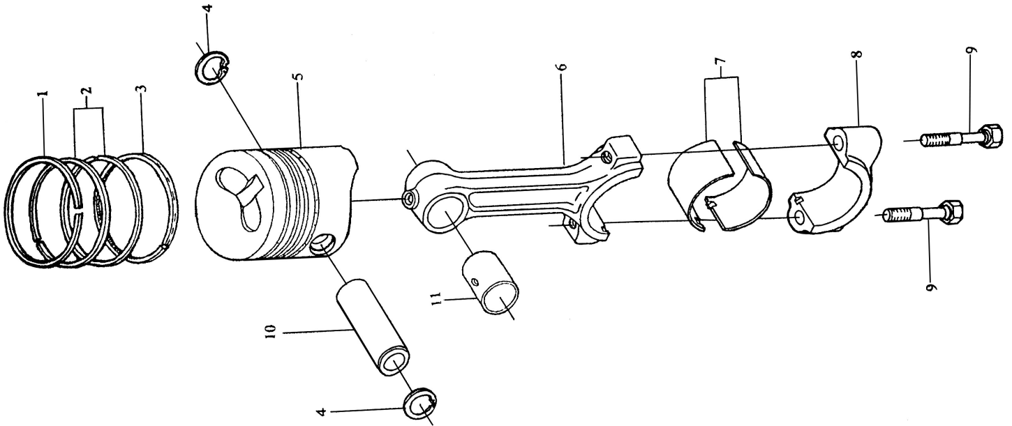
Fig. 4 Piston-connecting Rod Assy(385)
