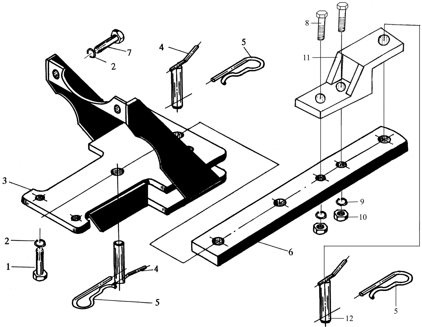
Fig. 6 Pendulum Drawbar
