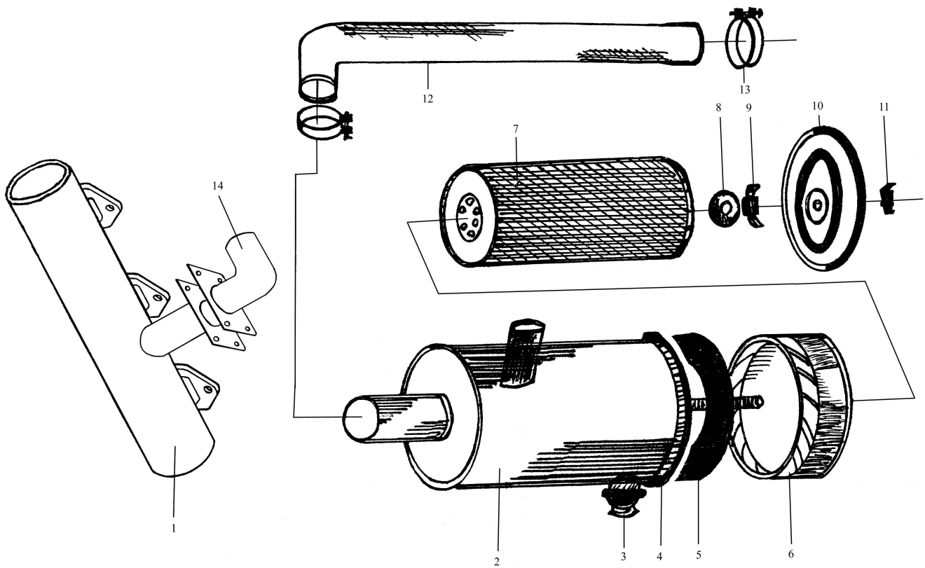
Fig. 7 Intake Pipe Assy and Air Filter Assy(Y385T-1)
