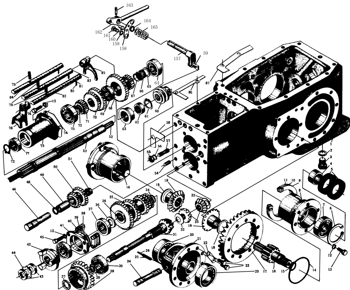
Fig.8 Drive Gearbox (Double Speed) III
