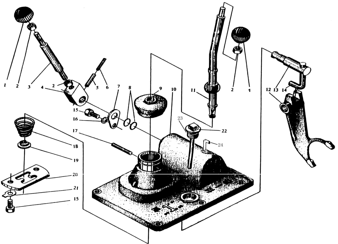
Fig. 9 Drive Gearbox Cover
