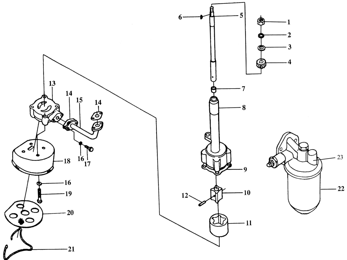
Fig. 9 Lubricating System Assy(Y385)
